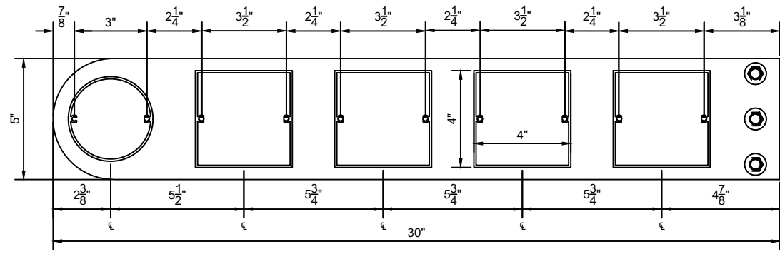
4" x 4" Tubular Sunshade
