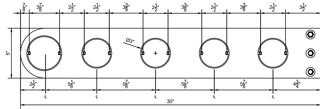
3" Ø Tubular Sunshade
