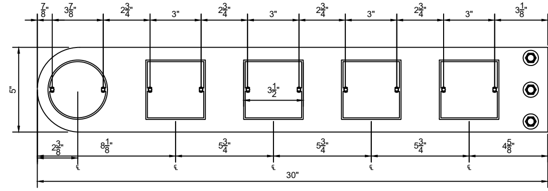
3 1/2" x 3 1/2" Tubular Sunshade
