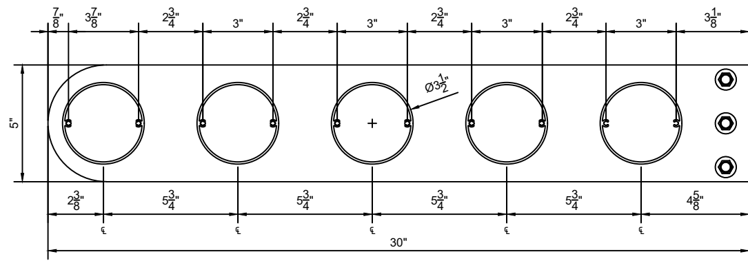
3 1/2" Ø Tubular Sunshade
