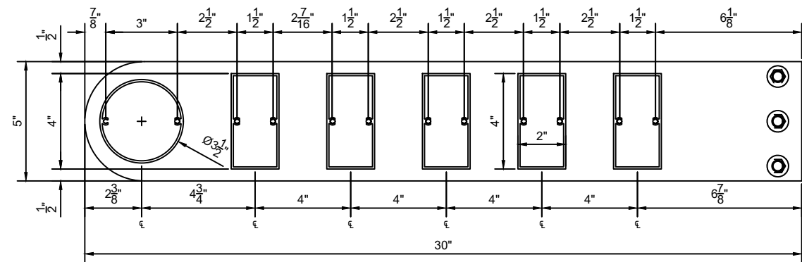
2" x 4" Tubular Sunshade
